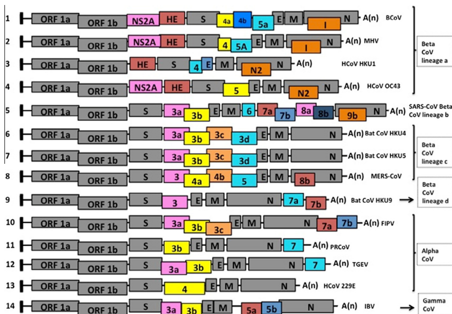
Fig. 5. Genome organization of members of Betacoronavirus lineages a–d, as well as of the genera Alphacoronavirus and Gammacoronavirus, showing structural and accessory genes downstream of the orf1a/1b gene. The 5' leader sequence (black box), open reading frames (ORFs 1a, 1b) encoding components of the replication/transcription complex, the genes encoding the structural proteins spike (S), membrane (M), envelope (E), and nucleocapsid (N) are also indicated in gray. Interspersed between (or within) them are the genes coding for putative accessory proteins (not drawn to scale). The following coronavirus genomes are illustrated (GenBank accession numbers in brackets): (1) Bovine coronavirus (NC_003045), (2) Mouse Hepatitis Virus (AC_000192), (3) Human coronavirus HKU1 (NC_006577), (4) Human coronavirus OC43 (NC_005147), (5) Severe Acute Respiratory Syndrome coronavirus (NC_004718), (6) Tylonycteris bat coronavirus HKU4 (NC_009019), (7) Pipistrellus bat coronavirus HKU5 (NC_009020), (8) MERS coronavirus (NC_019843), (9) Roussetus bat coronavirus HKU9 (NC_009021), (10) Feline infectious peritonitis virus (NC_002306), (11) Porcine respiratory coronavirus (DQ811787), (12) Transmissible gastroenteritis virus (DQ811788), (13) Human coronavirus 229E (NC_002645), (14) Infectious Bronchitis Virus (NC_001451).
