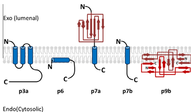
Fig. 3. Schematic diagram showing the known topological and structural features of SARS-CoV accessory proteins. N-terminus (N) and C-terminus (C) are indicated. \alpha -Helices are represented by blue columns and \beta -strands are represented by red arrows. The topological or structural features of p3b, p8a, and p8b are not well understood. Ribbon diagrams for p7a and p9b are adapted from Nelson et al. (2005) and Meier et al., 2006, respectively.
