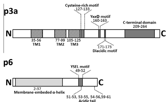
Fig. 2. Schematic diagram showing motifs and domains within SARS-CoV accessory proteins p3a and p6. TM, transmembrane domain.
