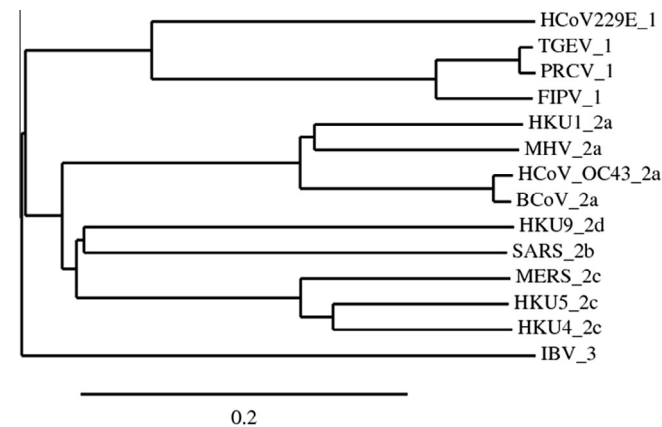
Fig. 4. Phylogenetic analysis of coronaviruses based on pp1ab using Kalign multiple sequence alignment and TreeDyn tree viewer (Chevenet et al., 2006; Lassmann and Sonnhammer, 2005). Next to the branch, the virus name is indicated, along with the previously defined viral lineages, i.e. group 1 for Alphacoronavirus members, 2a, 2b, 2c, 2d for Betacoronavirus members, and 3 for the member of the genus Gammacoronavirus . Scale bar indicates nucleotide substitutions per site.
